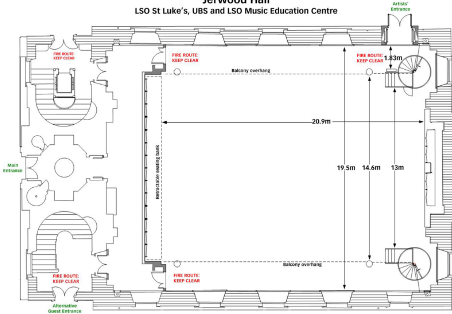
Clear floor plan with dimensions
